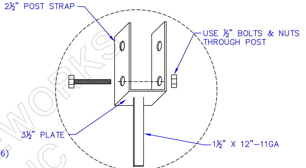
BRACKET ATTACHMENT DETAIL
